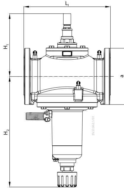
AB-PM DN 65-100
