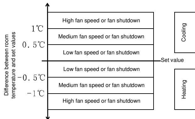
Figure 1 Automatic fan speed control algorithm
